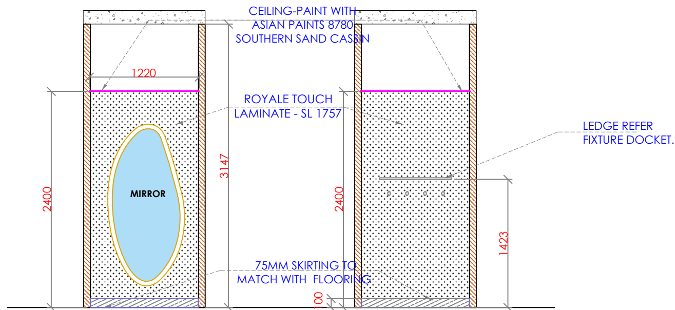
1 SECTION S1 Scale: NTS
